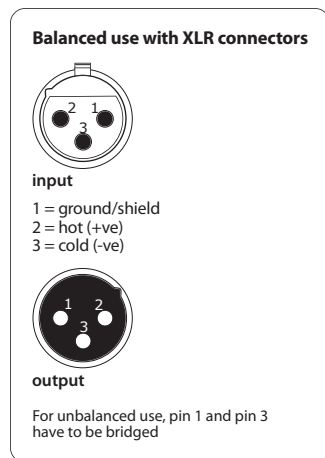
Fig. 4.2: XLR connections
