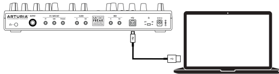
MicroFreak-Computer connection
