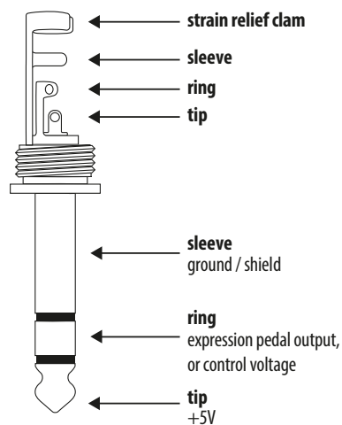
Expression or Control Voltage Connection Cable Wiring
