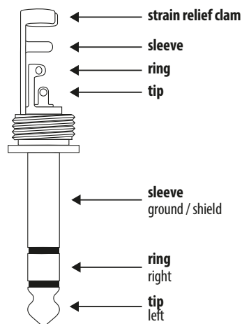
Headphones Connection Cable Wiring
