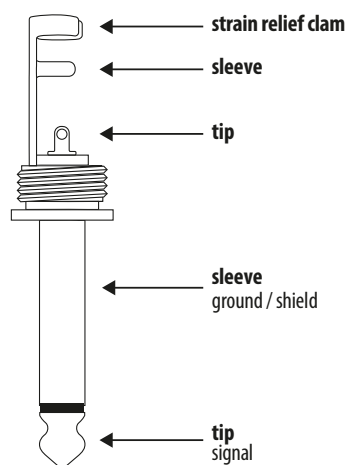
Un-Balanced Connection Cable Wiring
