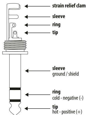
Balanced Connection Cable Wiring
