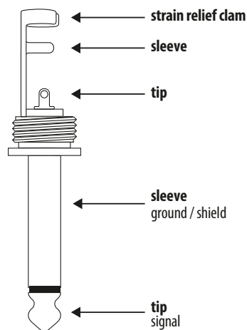
Sustain Connection Cable Wiring
